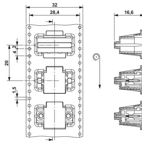
Dimensioned drawing
