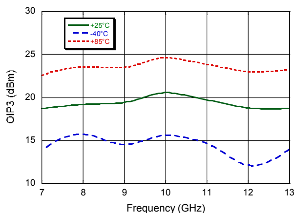
Output IP3 vs. Temperature for V_{DD} = 5\text{ V}
