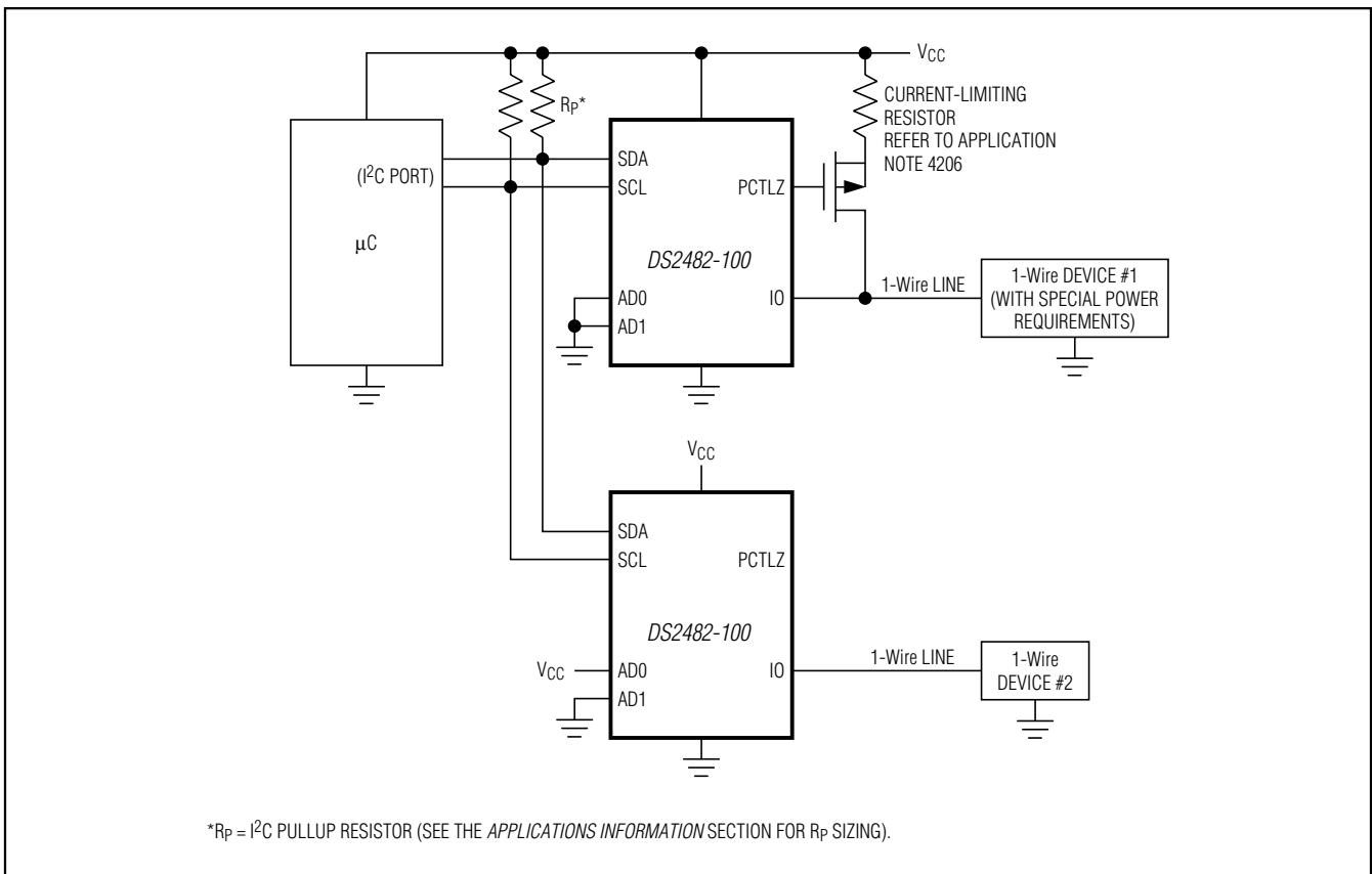
Figure 10. Application Schematic
