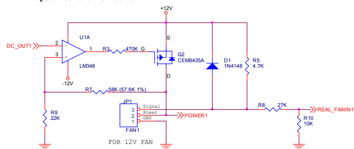
PWM FAN Speed control circuit
