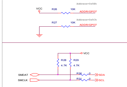
I2C Slave Address Select circuit
