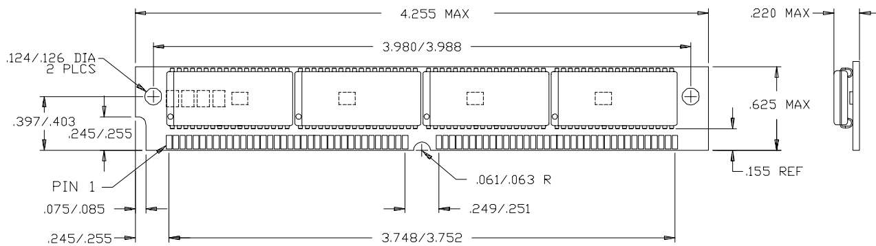
72-Pin Plastic ZIP Module PZ11
