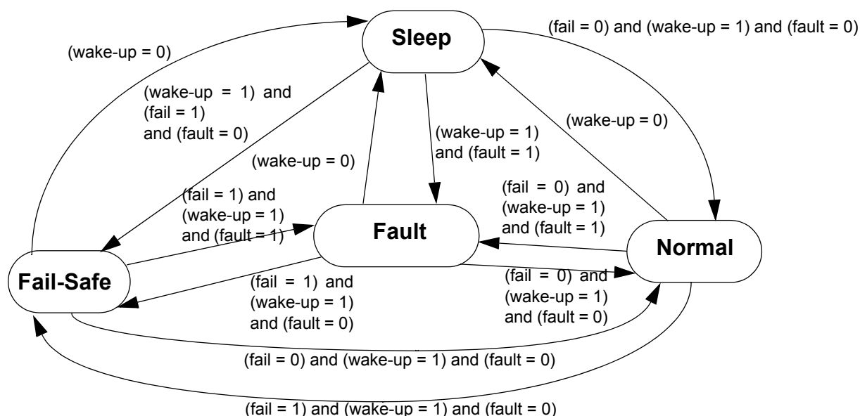
Figure 12. Operating Modes
