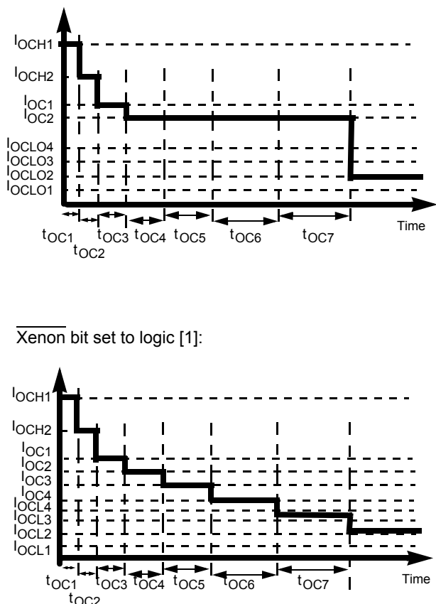
Figure 14. Overcurrent Profile Depending on Xenon Bit
