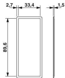
Side element (front and back)
