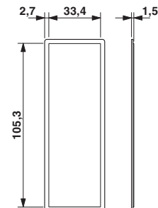
Cover element
