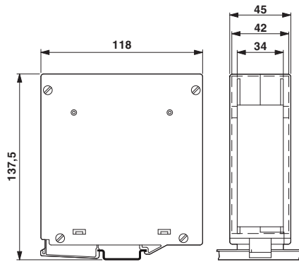
Dimensioned drawing
