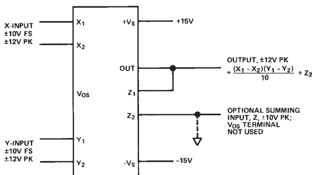
Figure 5. Basic Multiplier Connection
