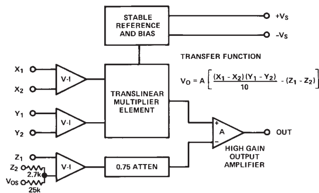
Figure 4. AD632 Functional Block Diagram
