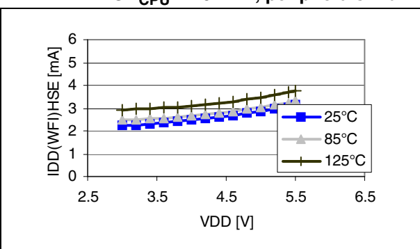
Figure 15. Typ. I_{DD(WFI)HSE} vs. V_{DD} @ f_{CPU} = 16 MHz, peripherals = on
