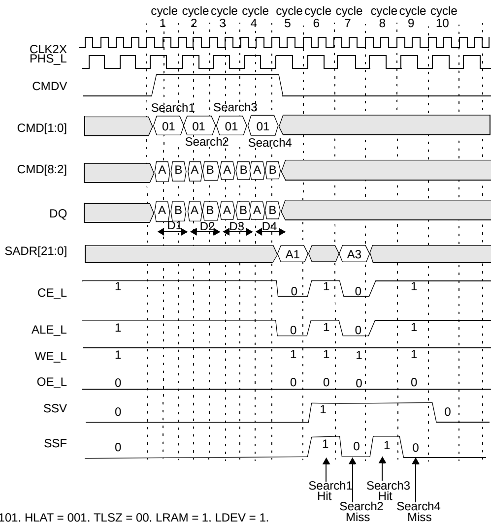
Figure 13-23. Timing Diagram for 136-bit Search (One Device)
