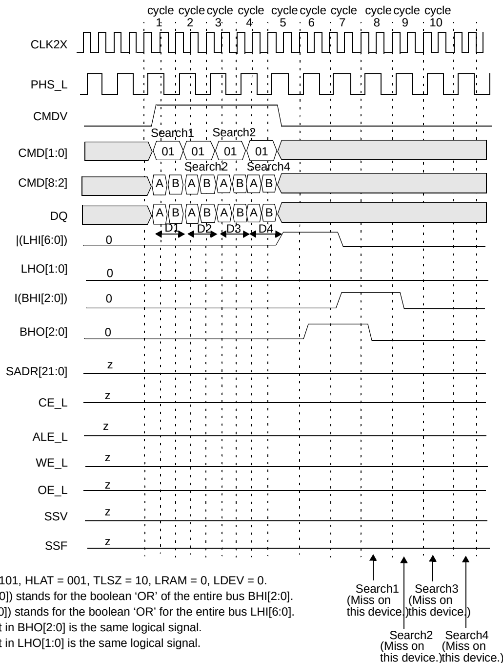
Figure 13-42. Timing Diagram for Devices Below the Winning Device in Block Number 3 Except Device Number 30 (the Last Device)
