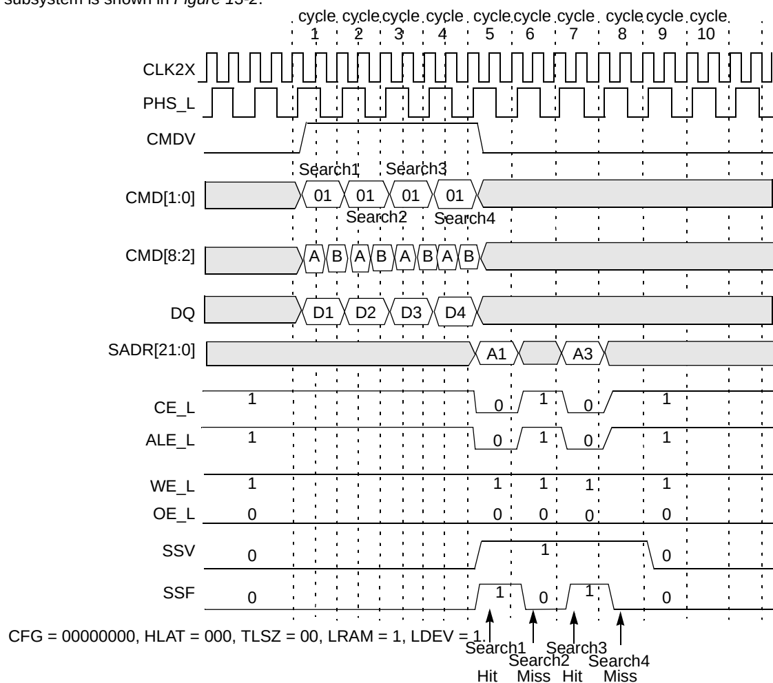
Figure 13-1. Timing Diagram for 68-bit Search in \times 68 Table (One Device)
