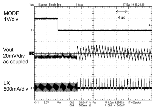
Fig.8 Mode Change Response MODE High to Low
