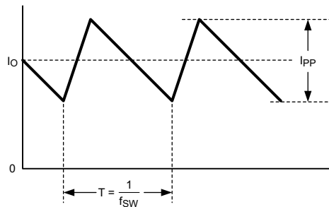
Figure 7-2. Inductor Current
