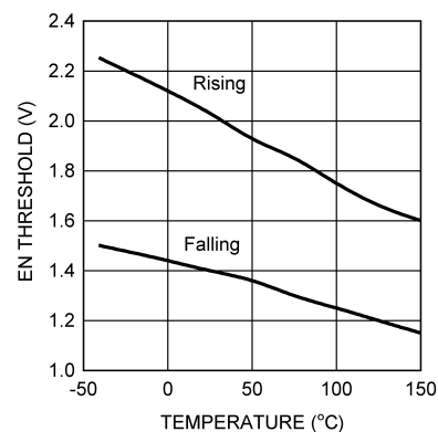
Figure 5-8. EN Input Threshold vs Temperature
