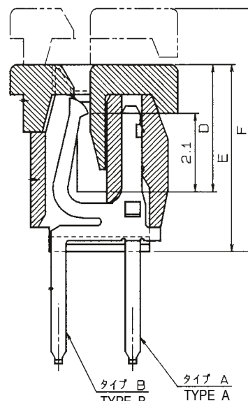
SECT. W-W
