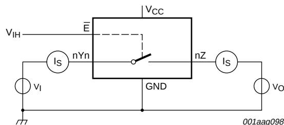
Fig 6. Test circuit for measuring OFF-state leakage current
