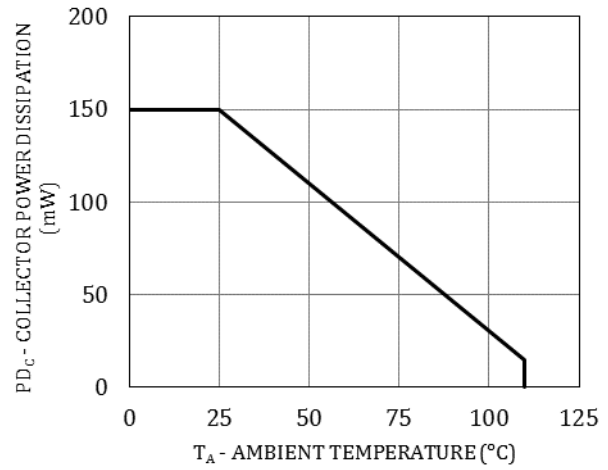
Figure 2. Collector Power Dissipation vs. Ambient Temperature
