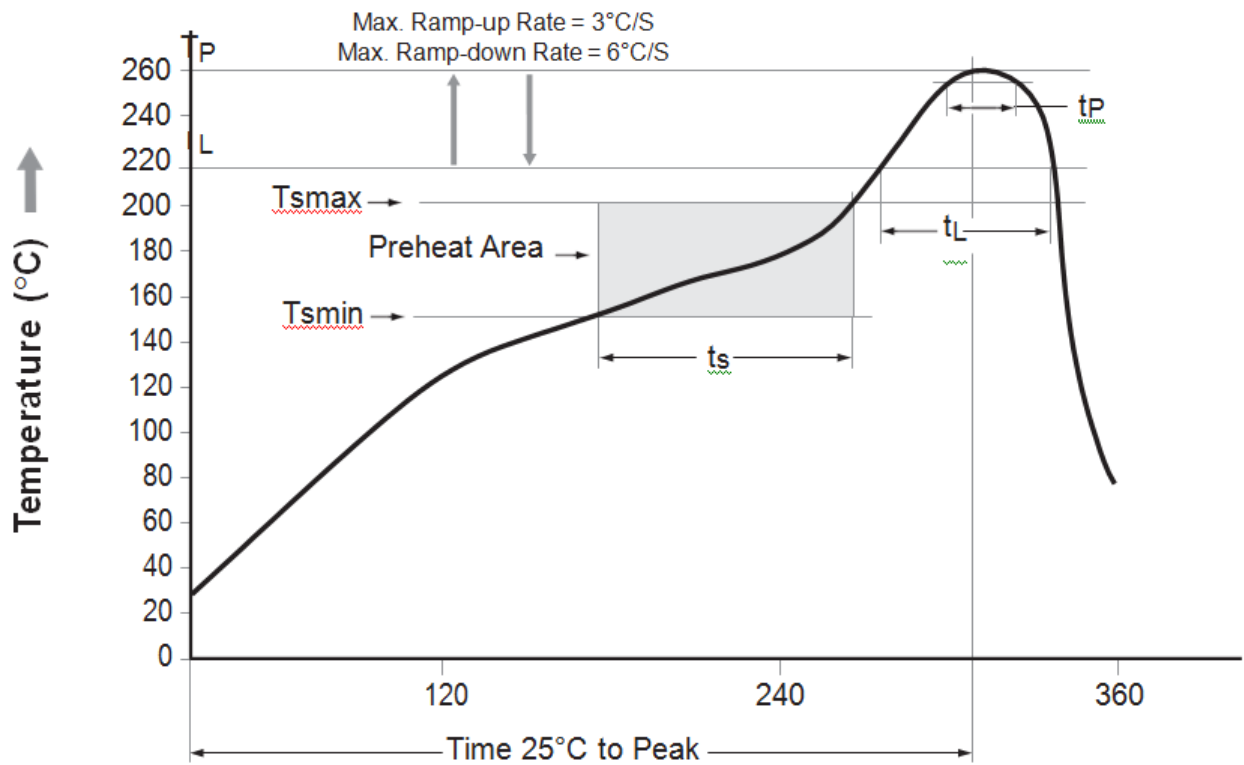
Figure 12. Reflow Profile
