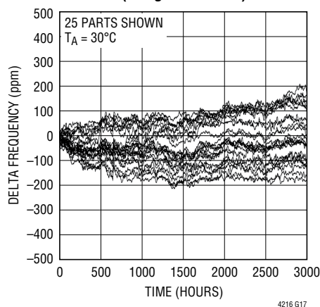
Typical Frequency Error vs Time (Long-Term Drift)
