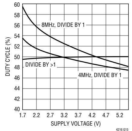
Typical Output Duty Cycle vs Supply and Divide Ratio
