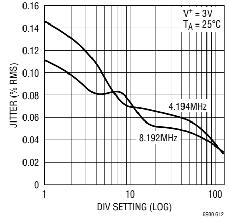
Typical Jitter vs Divider Setting
