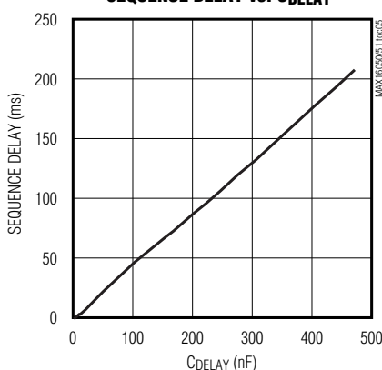
SEQUENCE DELAY vs. CDELAY
