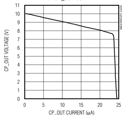
CP_OUT VOLTAGE vs. CP_OUT CURRENT
