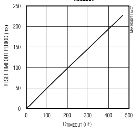
RESET TIMEOUT PERIOD vs. CTIMEOUT
