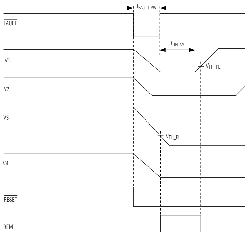
Figure 3. Sequencing Timing Diagram During a System Fault
