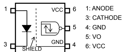
Pin Configuration (Top View)
