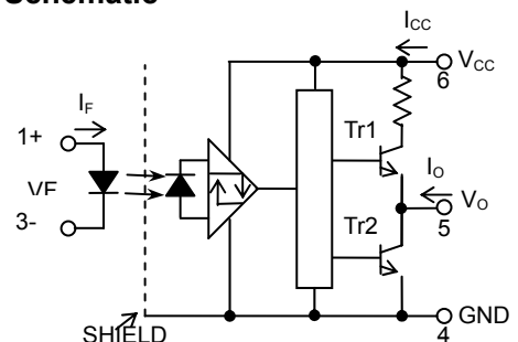
Schematic
