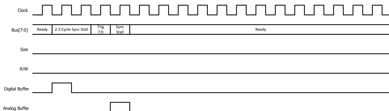
Figure 10-8. ADC Trigger
