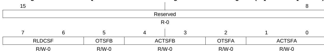
Figure 7-101. Action-Qualifier Software Force Register and Mirror Register (AQSFRC / AQSFRCM)
