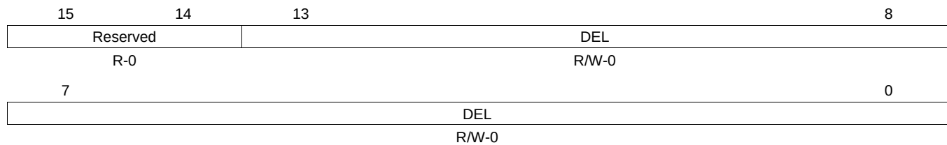
Figure 7-105. Dead-Band Generator Rising Edge Delay and Mirror Register (DBRED / DBREDM)
