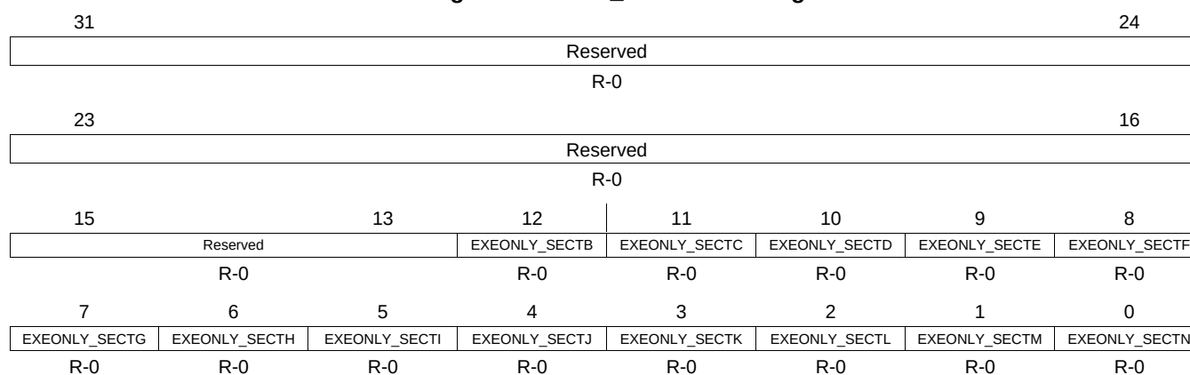
Figure 1-145. Z2_EXEONLYR Register
