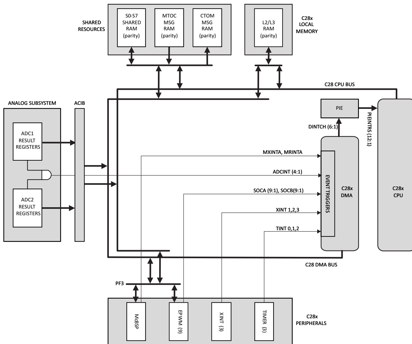
Figure 11-1. DMA Block Diagram
