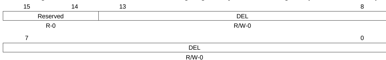
Figure 7-106. Dead-Band Generator Falling Edge Delay and Mirror Register (DBFED / DBFEDM)
