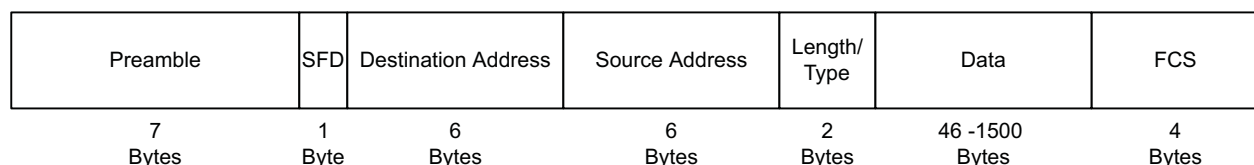
Figure 19-3. Ethernet Frame
