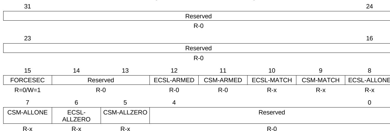
Figure 1-138. Z1_CSMCR Register
