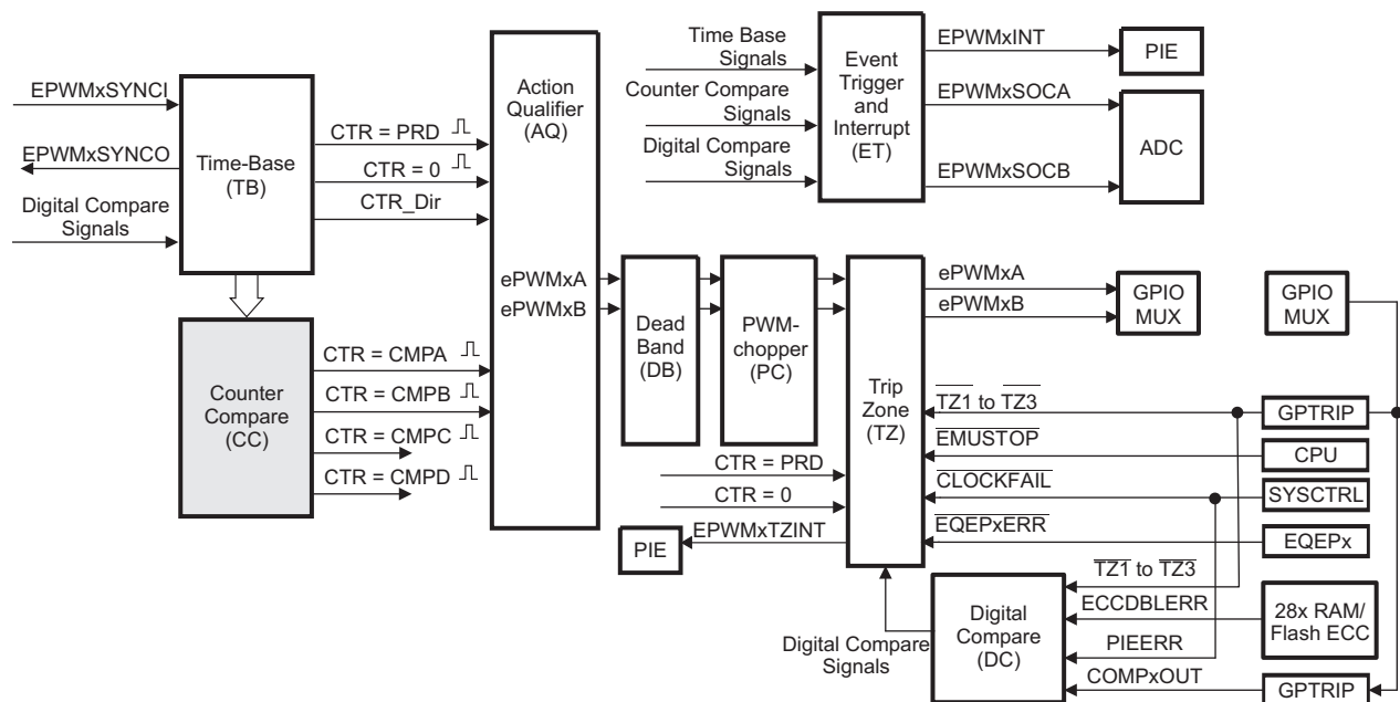
Figure 7-12. Counter-Compare Submodule
