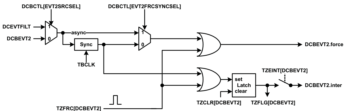
Figure 7-52. DCBEVT2 Event Triggering
