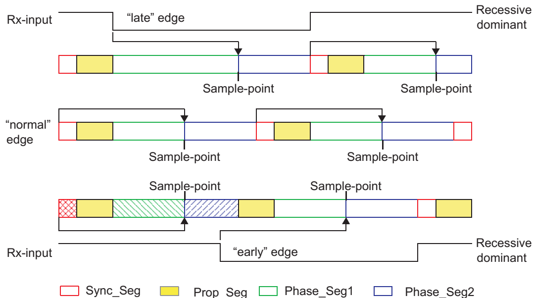
Figure 23-13. Synchronization on Late and Early Edges
