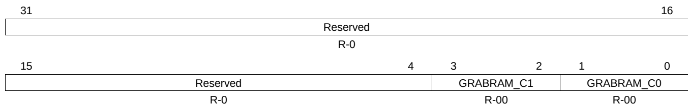
Figure 1-141. Z1_GRABRAMR Register
