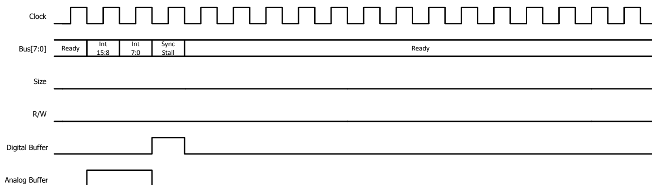
Figure 10-9. ADC Interrupt
