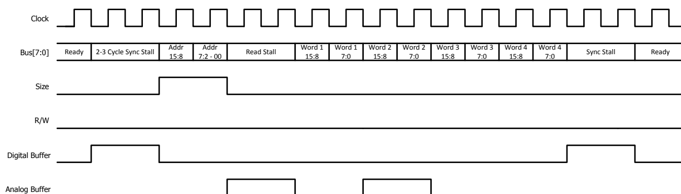
Figure 10-7. 64-bit Read
