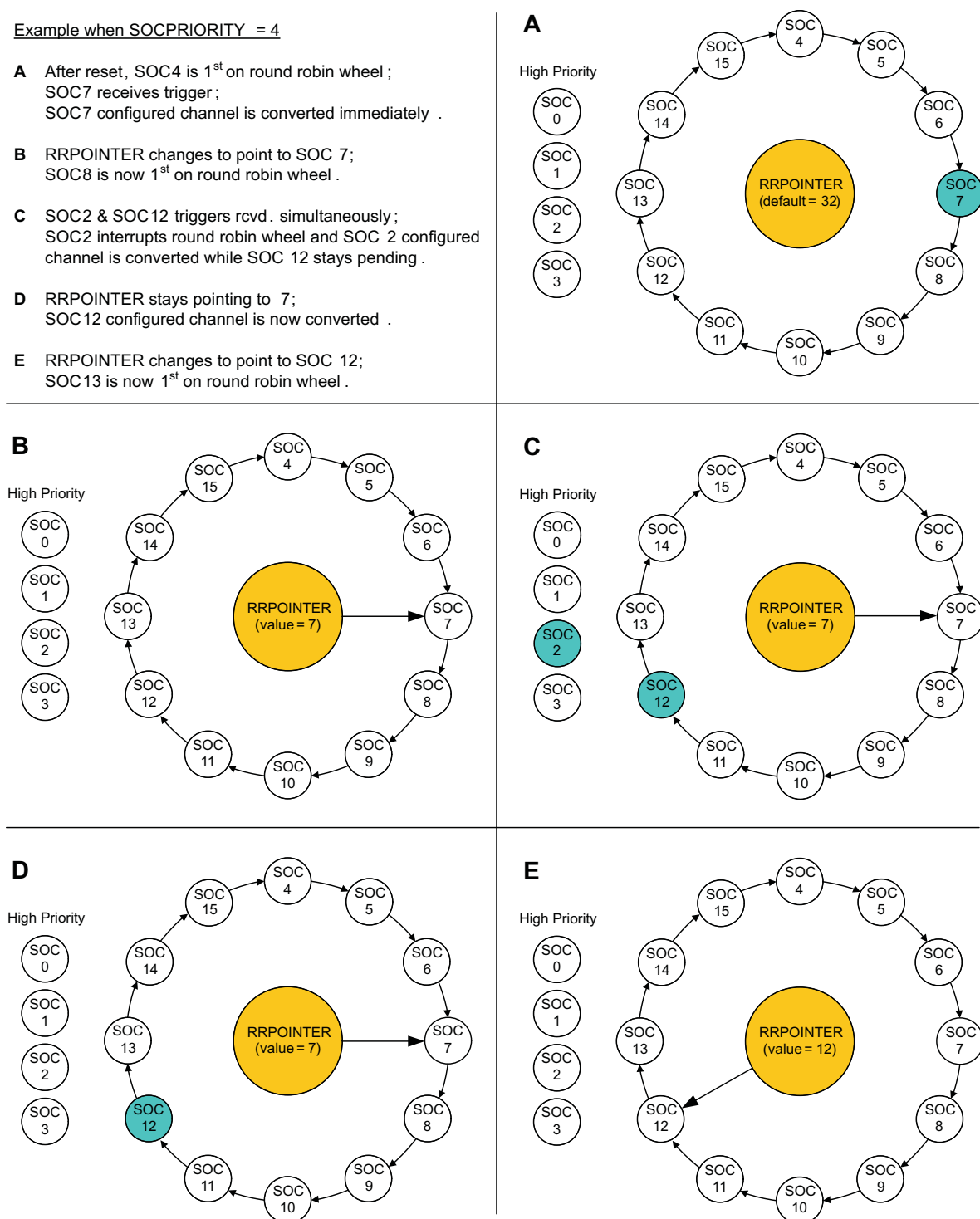
Figure 10-15. High Priority Example
