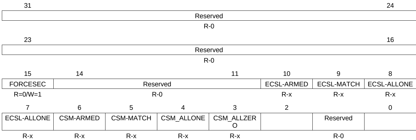
Figure 1-151. CSMCR Register
