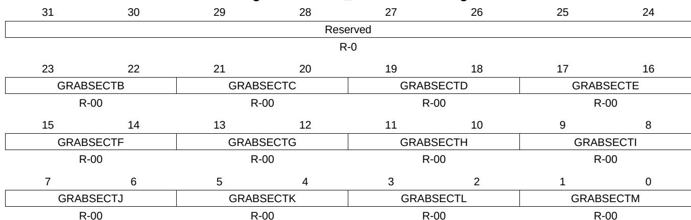
Figure 1-142. Z2_GRABSECTR Register
