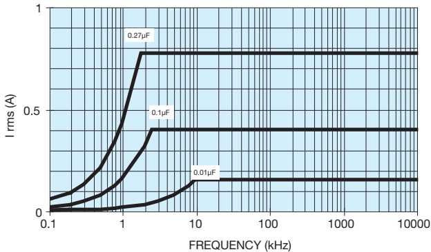
630 Vdc / 250 Vac
