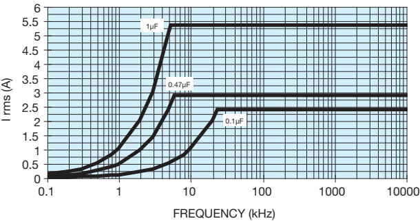
250 Vdc / 160 Vac
