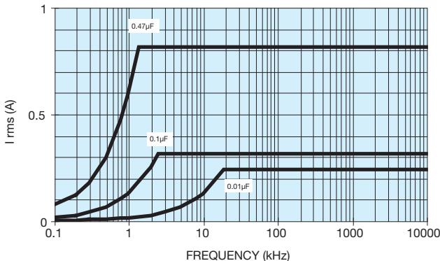
400 Vdc / 200 Vac
