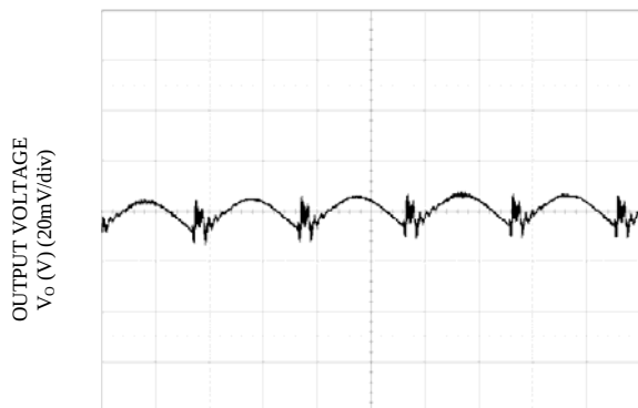
TIME, t (1 \mu s/div) Vo=0.69V, Io = Io,max
