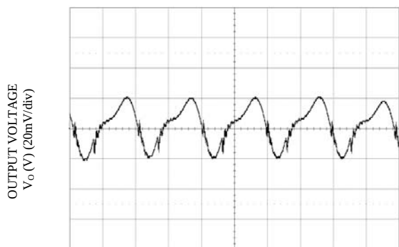
TIME, t (1 \mu s/div) Vo=3.3V, Io = Io,max
