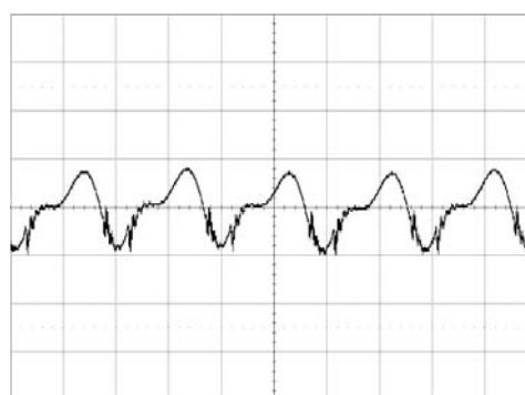
TIME, t (1 \mu s/div) Vo=2.5V, Io = Io,max
