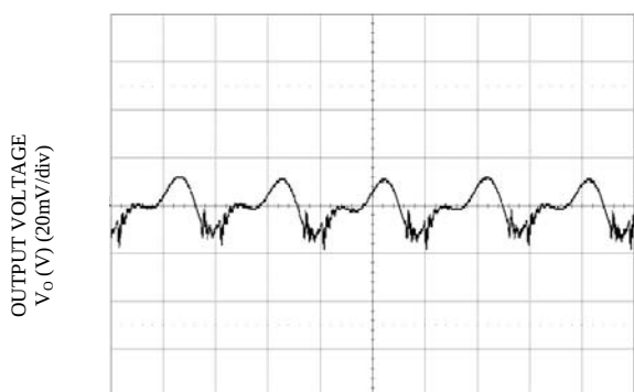
TIME, t (1 \mu s/div) Vo=1.8V, Io = Io,max
