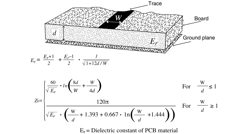
Figure 27: Microstrip Formulas
