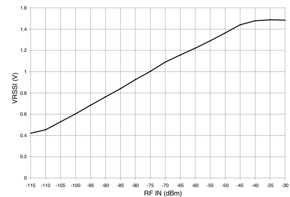
Figure 7: RSSI Curve
