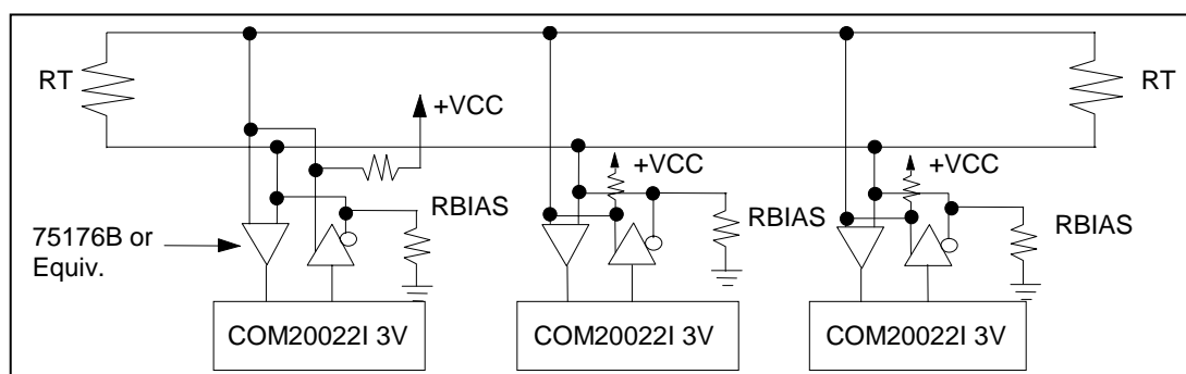
Figure 5.8 - COM20022I 3V Network Using RS-485 Differential Transceivers
