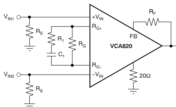
Figure 81. Differential Equalizer
