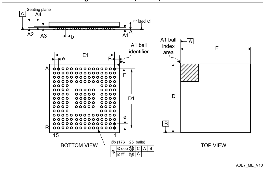
Figure 89. UFBGA(176+25) - Outline
