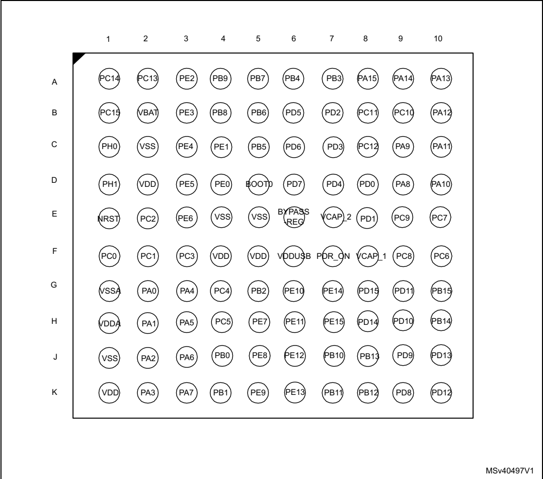
Figure 12. STM32F76xxx TFBGA100 ballout
