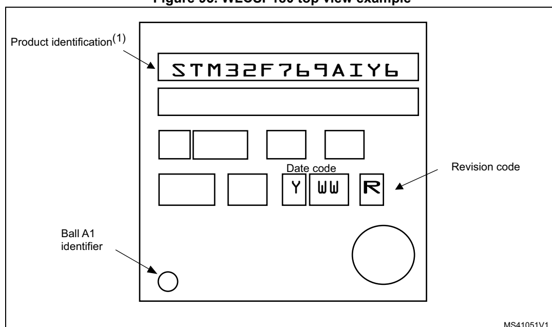
Figure 93. WLCSP180 top view example
