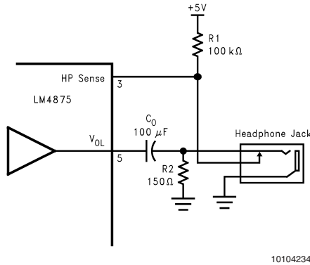
FIGURE 3. Headphone Circuit
