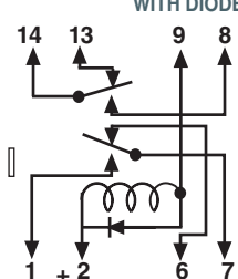
DPDT
