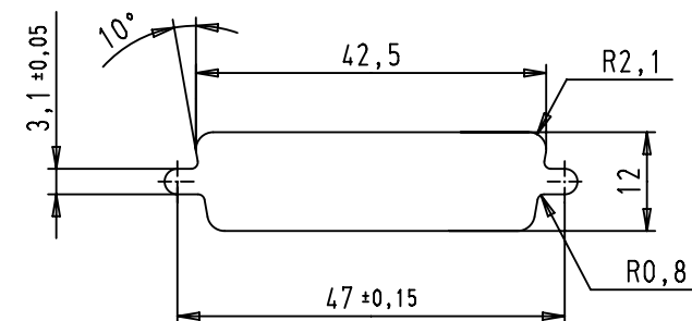
Panel cut out
