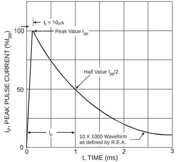
Figure 8 Pulse Waveform
