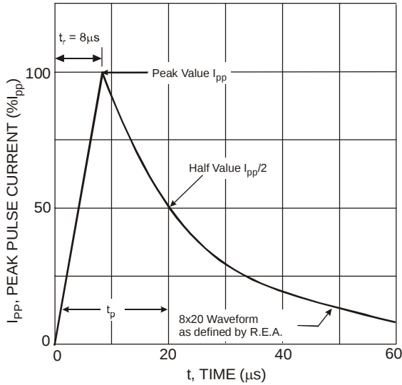
Figure 7 Pulse Waveform
