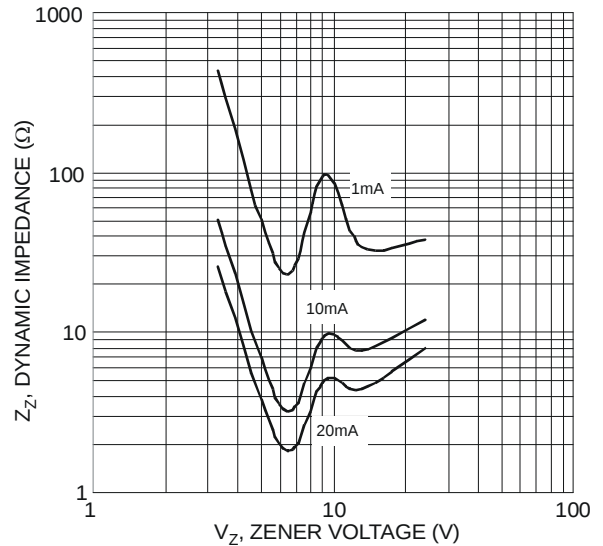
Figure 4 Effect of Zener Voltage
