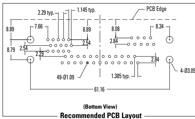
(Bottom View) Recommended PCB Layout
