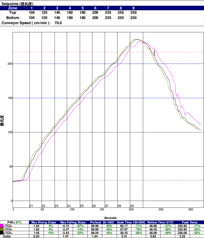
Figure 5 - Example solder reflow profile (AMWx36-E03 evaluation board)
