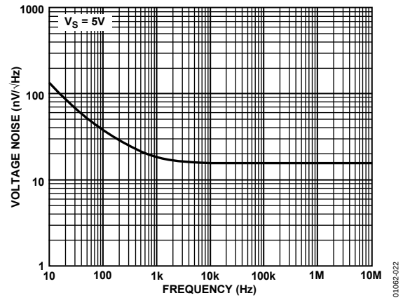
Figure 22. Input Voltage Noise vs. Frequency
