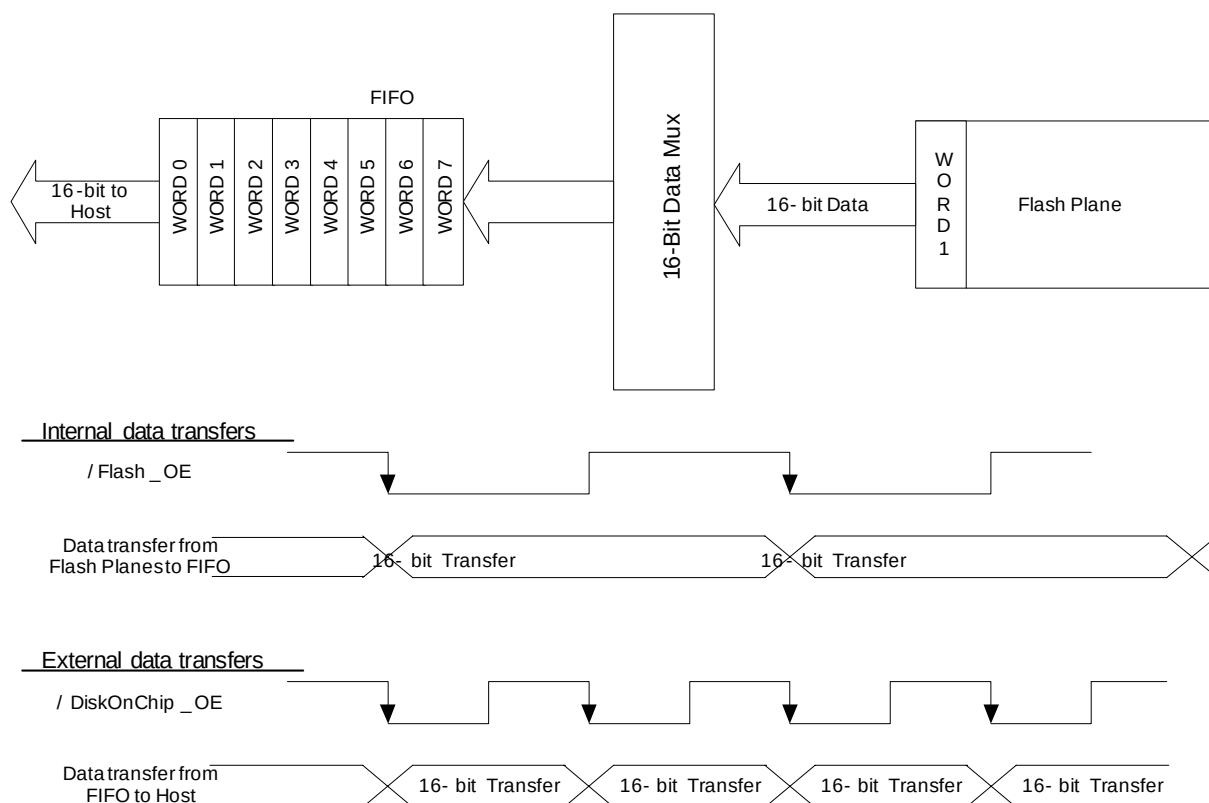
Figure 8: MultiBurst Operation
