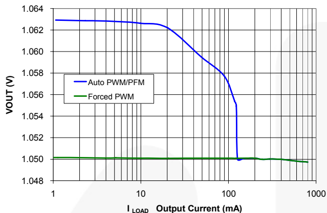
Figure 11. Load Regulation at V_{OUT} = 1.05V
