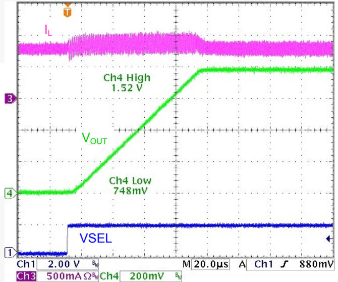
Figure 28. Multi-Step, Controlled DAC step (9.6mV/usec) DEF_Slew 6 (110), 800mA Load
