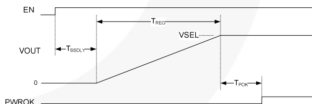
Figure 37. Soft Start Timing
