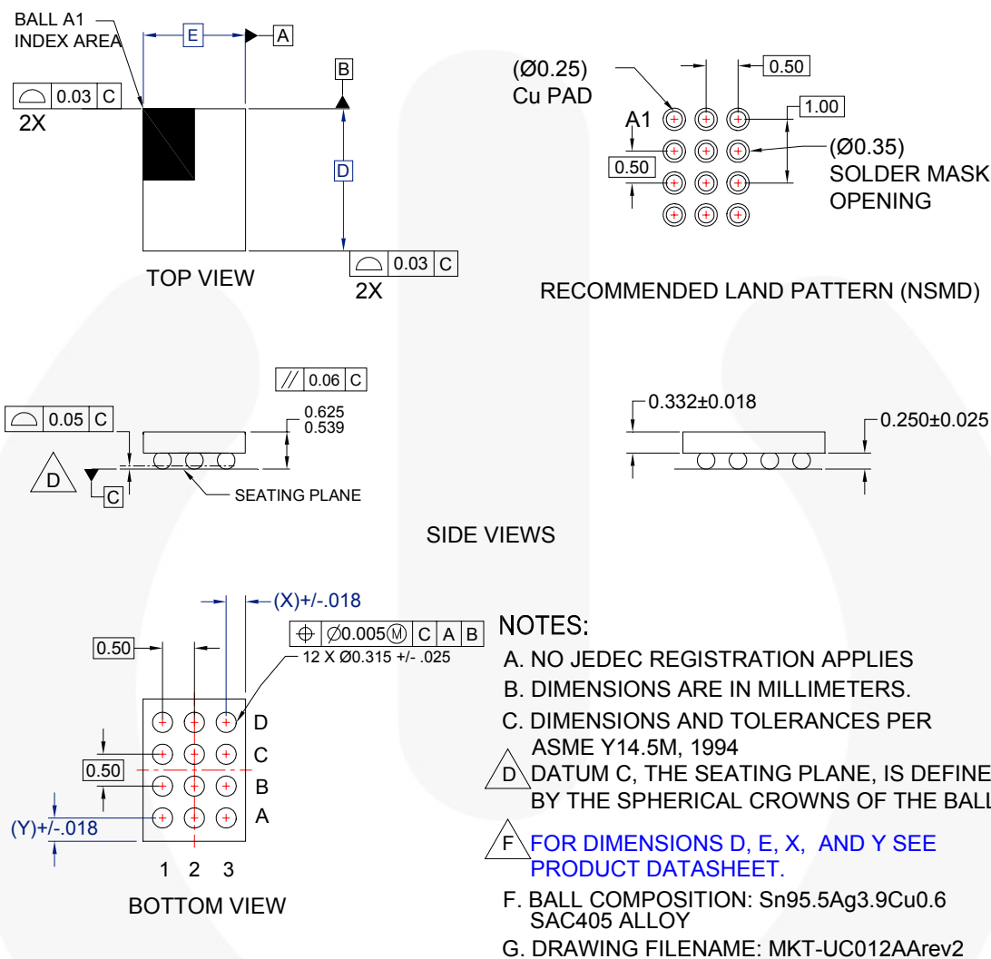
Figure 47. 12-Bump WLCSP, 0.5mm Pitch
