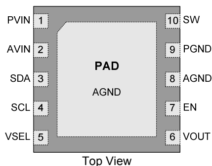
Figure 3. MLP10, 3x3mm
