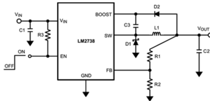
Figure 41. LM2738Y (550 kHz) V_{\text{BOOST}} Derived from V_{\text{OUT}} 12 V to 3.3 V / 1.5 A
