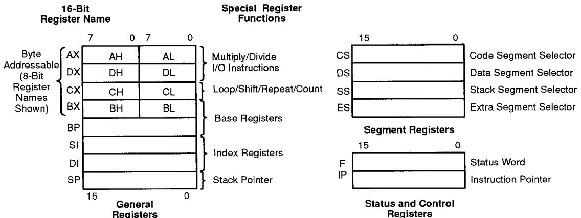
Figure 1. 80C186/C188 Register Set
