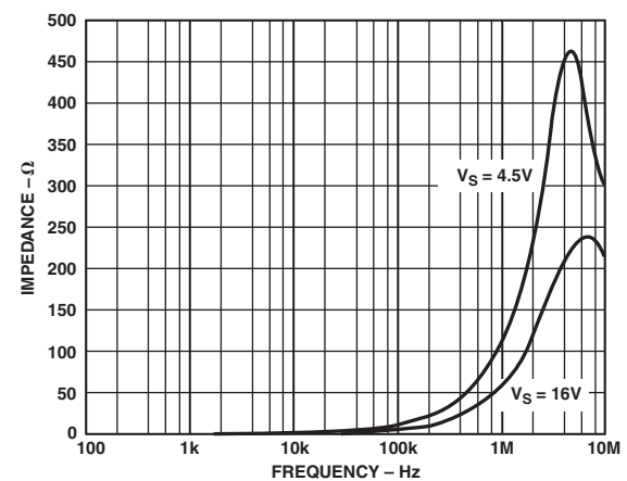
TPC 15. Closed-Loop Output Impedance vs. Frequency
