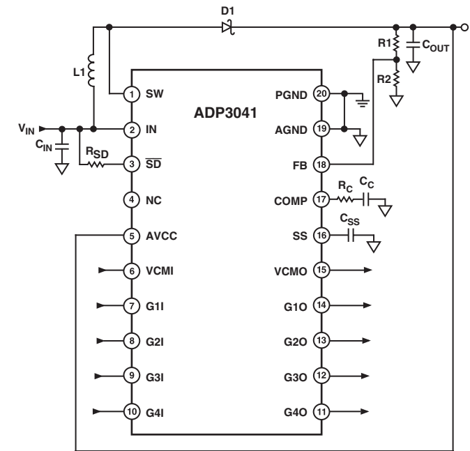
Figure 1. Typical Application
