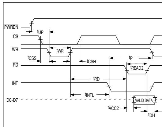
Figure 4. WR-RD Mode Timing ( t_{\text{RD}} > t_{\text{INTL}} ) (MODE = 1)
