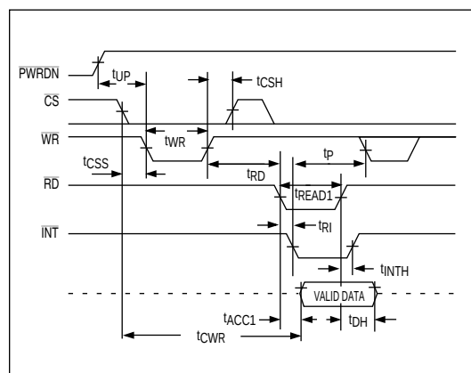
Figure 5. WR-RD Mode Timing ( t_{\text{RD}} < t_{\text{INTL}} ), Fastest Operating Mode (MODE = 1)
