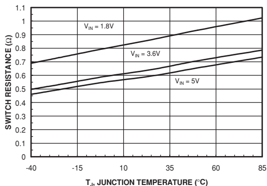
Figure 6. Switch Resistance vs. Temperature
