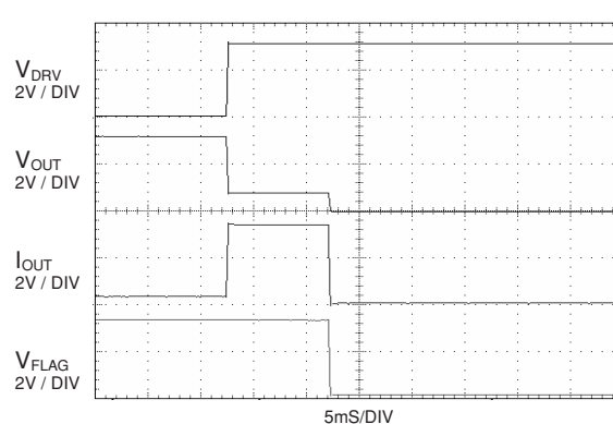
Figure 18. Fault Blanking Response
