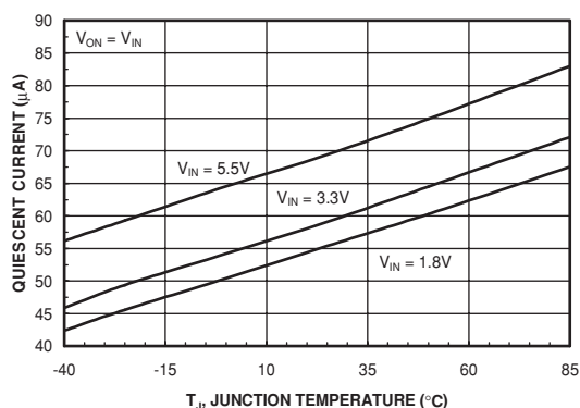
Figure 2. Quiescent Current vs. Temperature
