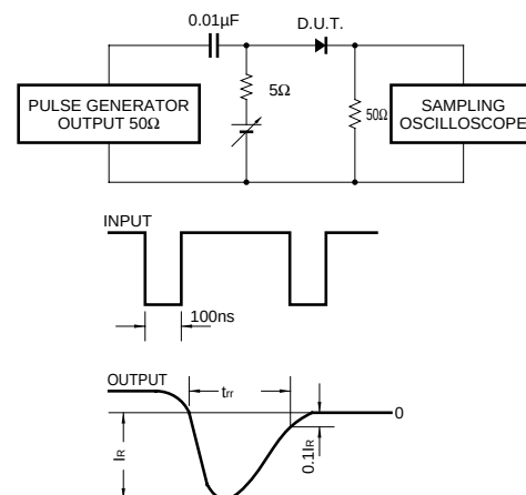
Fig. 8 Reverse recovery time ( t_{rr} ) measurement circuit
