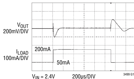
Load Transient 50mA to 200mA
