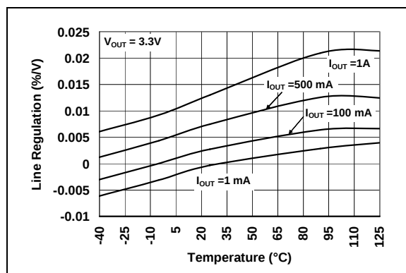
FIGURE 2-16: Line Regulation vs. Temperature (3.3V Fixed).
