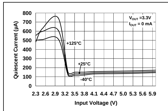
FIGURE 2-11: Quiescent Current vs. Input Voltage (3.3V Fixed).
