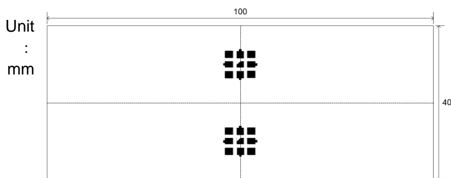
Fig.2 Testing board
