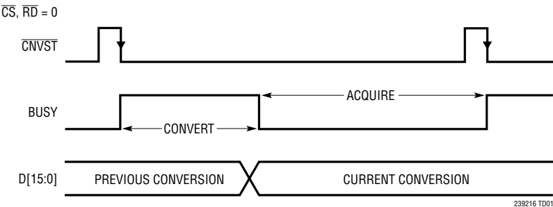
Conversion Timing Using the Parallel Interface
