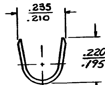
SECT B-B
