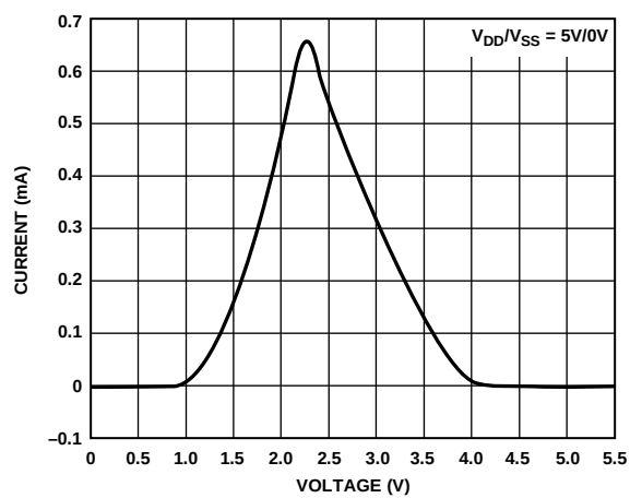
Figure 9. Supply Current ( I_{DD} ) vs. Digital Input Voltage
