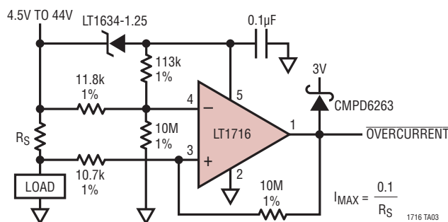
Overcurrent Flag
