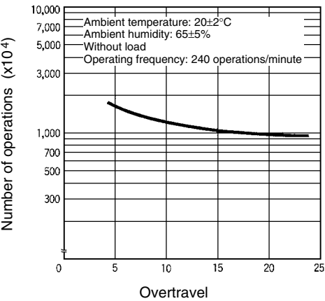
Mechanical Durability
