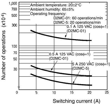
Electrical Durability
