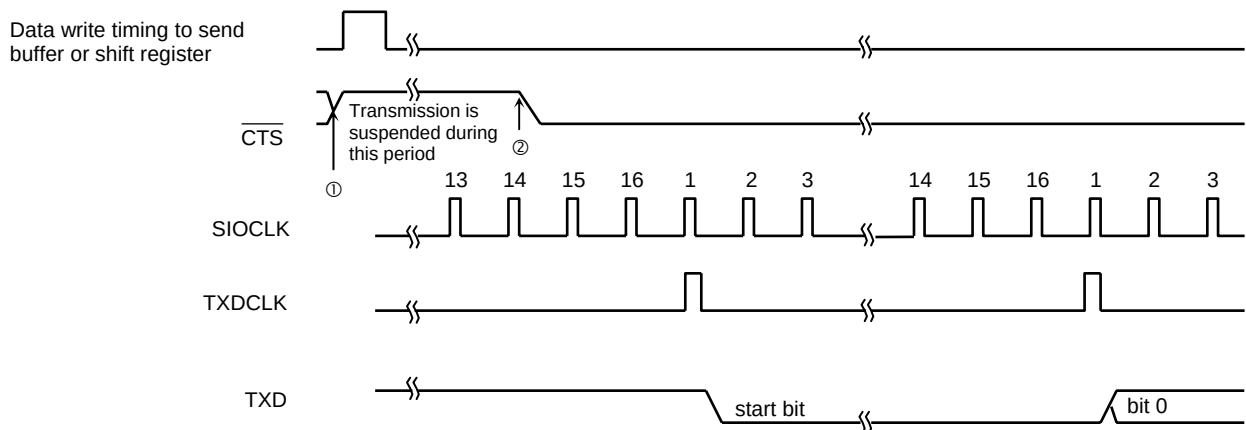
Fig. 13-6 Handshake Function
