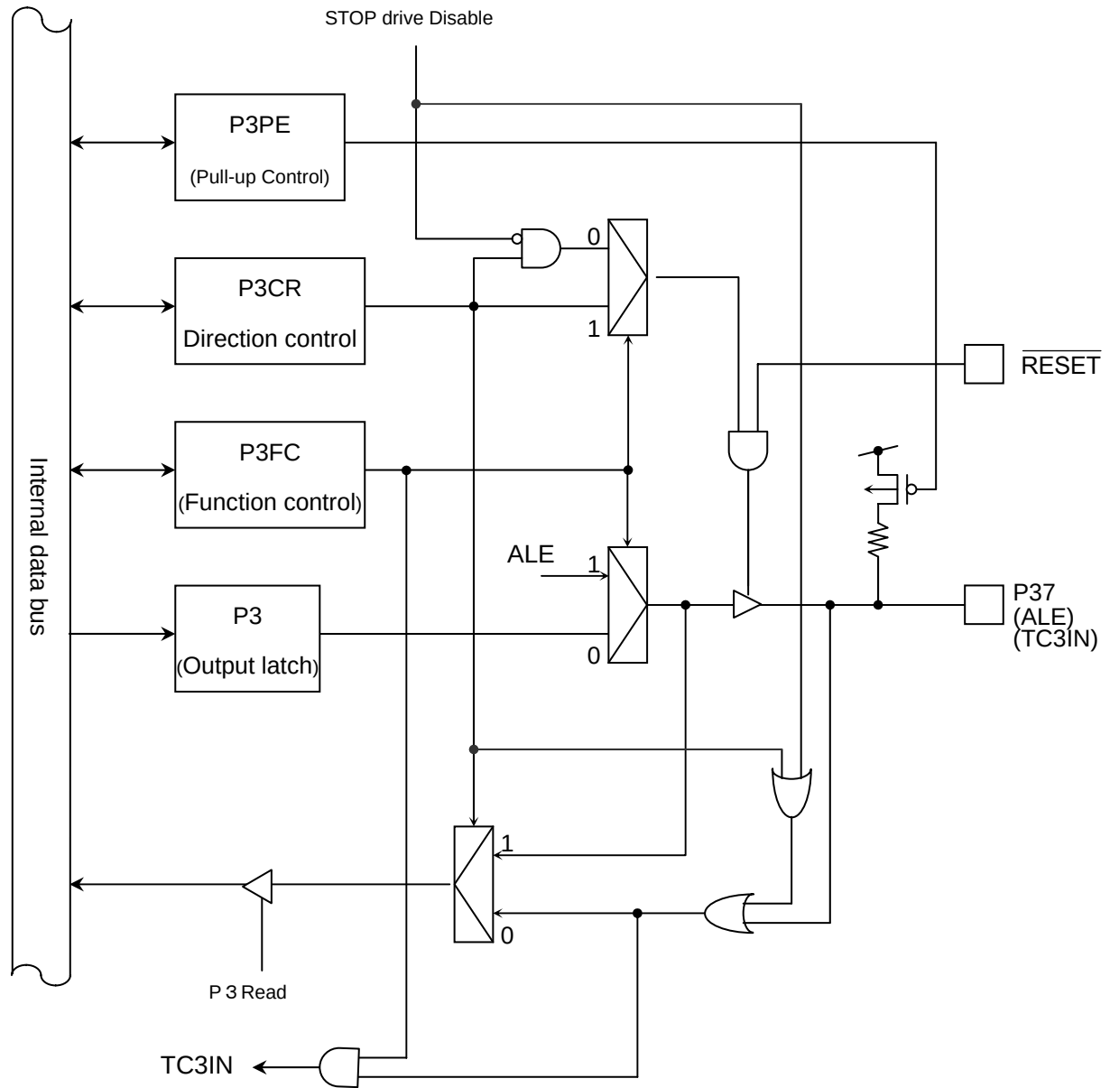
Fig. 7-8 Port 3 (P37)
