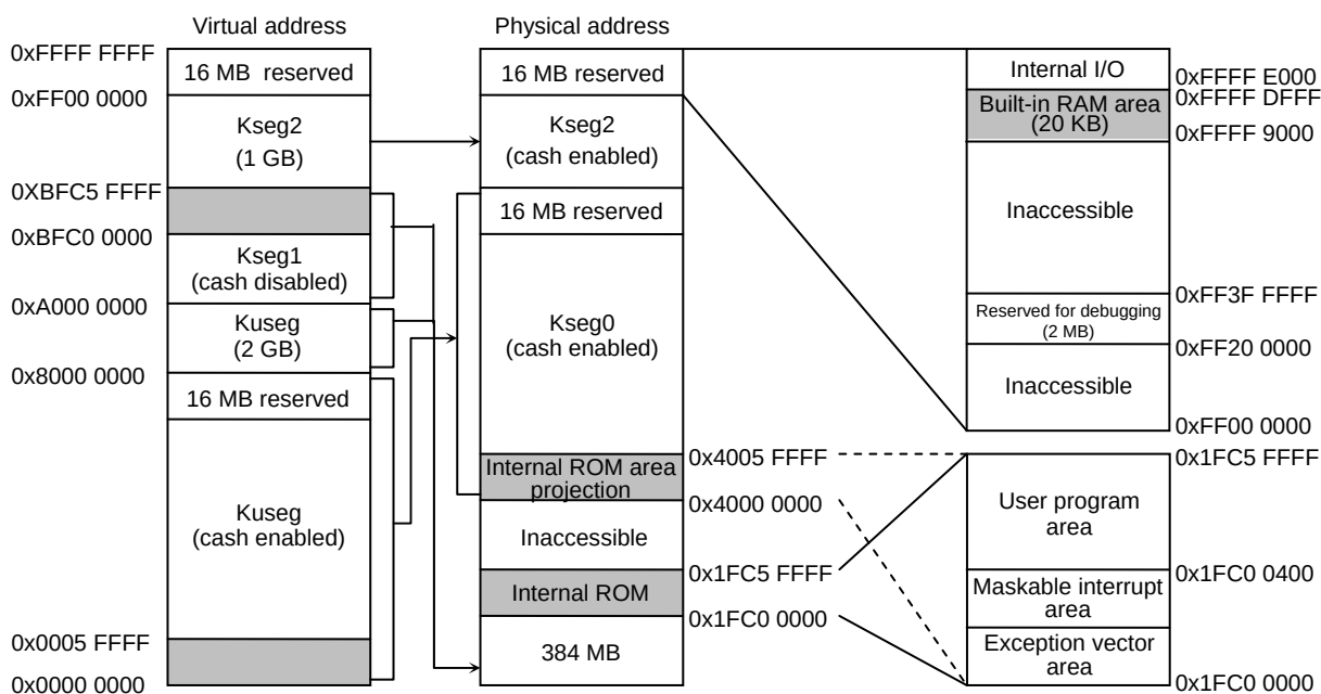
Fig. 4-2 Memory Map
