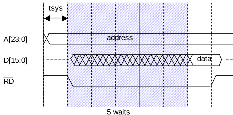
Fig. 8-4 Read Operation Timing Diagram (5 Waits Automatically Inserted)
