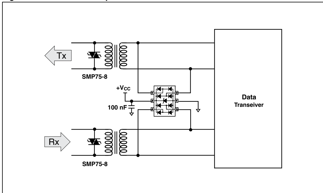
Figure 7. T1/E1/Ethernet protection
